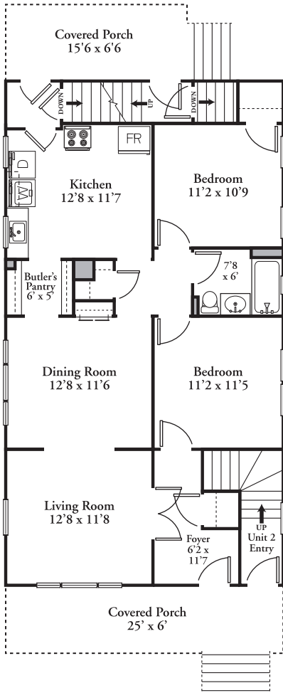
FIRST FLOOR - Unit 1
