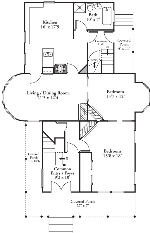
FIRST FLOOR - Unit 1 10'2" Ceiling Height
