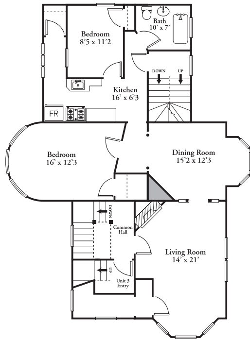
SECOND FLOOR - Unit 2 9'4" Ceiling Height
